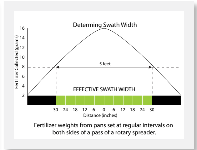
Figure 15. Determining swath width
